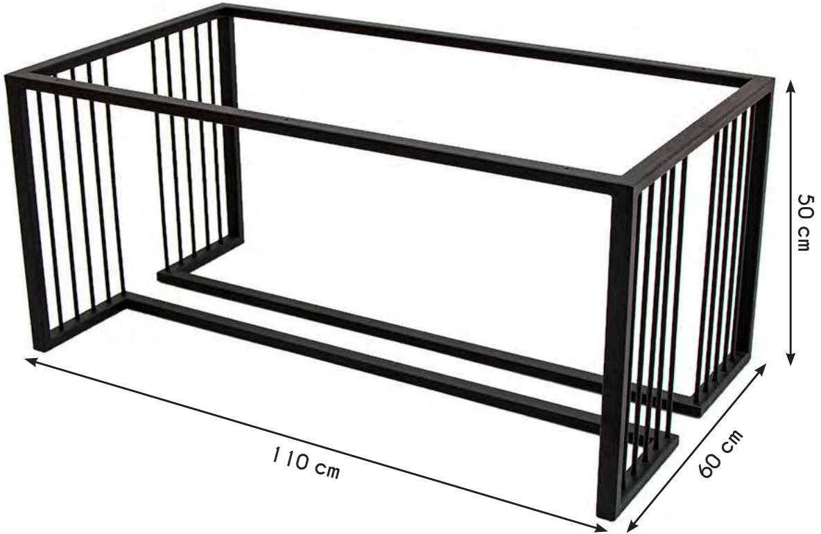
Orta Profil Sehpa Ayağı Middle Profile Coffee Table Leg
